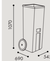
W0012 Rullkärl 190 liter
