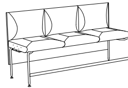
SA830 rak koppling (14) H 1030 SH 630 B 1910 D 650
