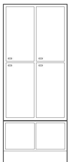
PF8/19-4 1932 x 800 x 372
