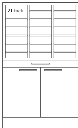
PS9/15 1580 x 910 x 372
