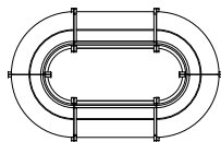
2xMEB120AVH, 4xMES90Y L3120 W1920 innermätt inner L1850 W650
